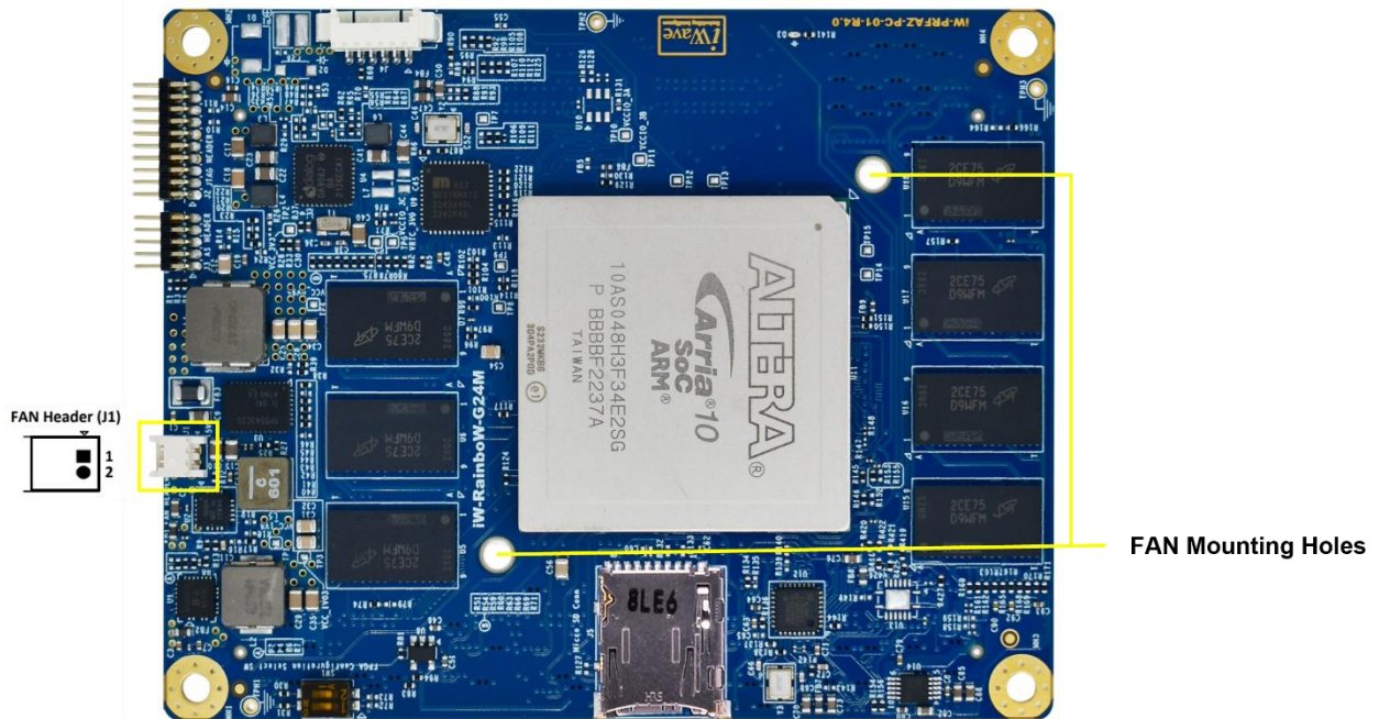
Figure 6: Fan Header
