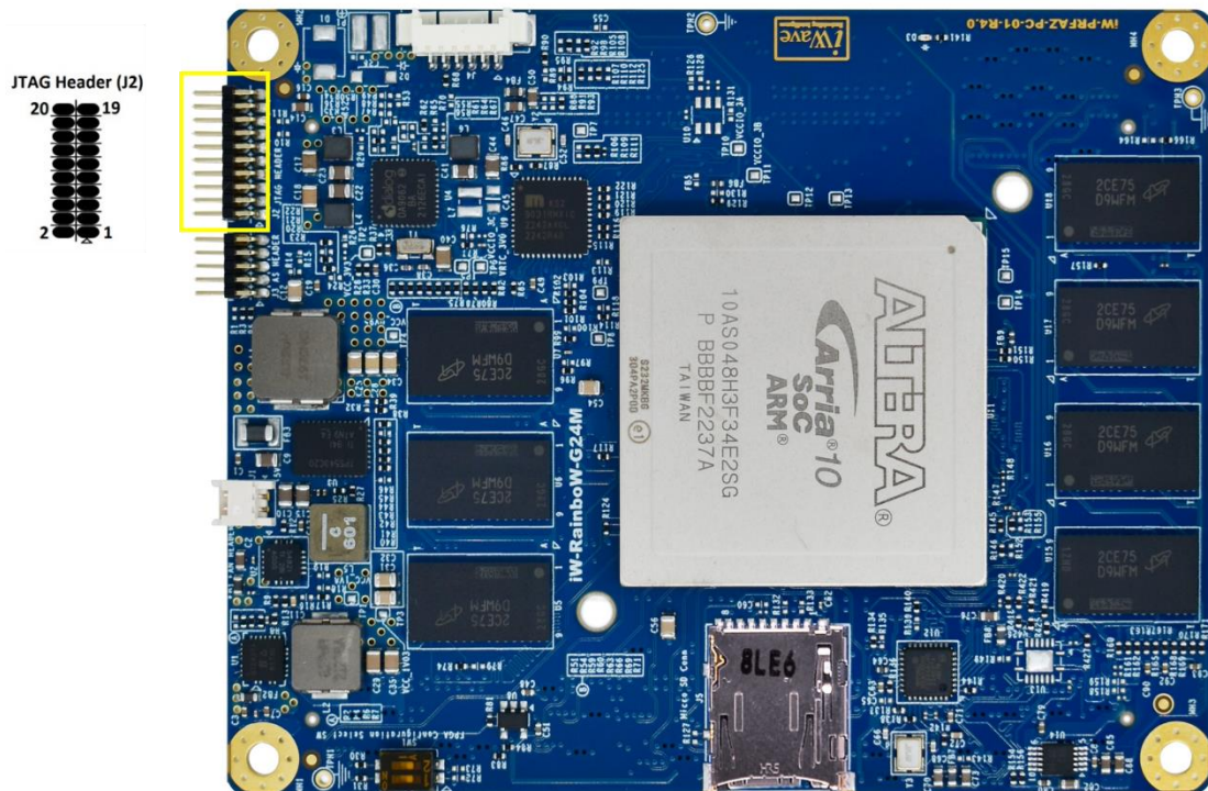
Figure 5: JTAG Header
