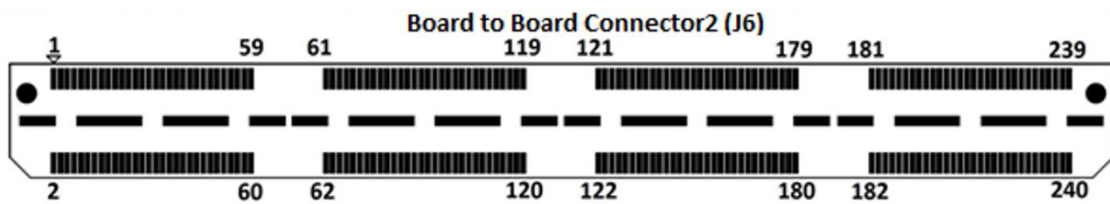
Figure 9: Board to Board Connector2
