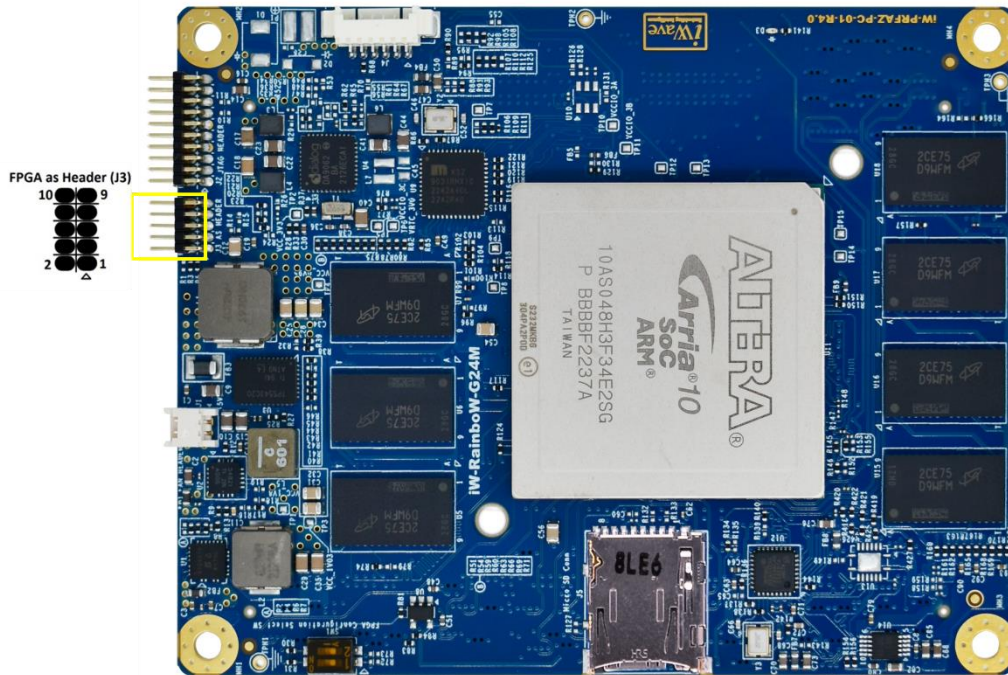
Figure 7: FPGA AS Header
